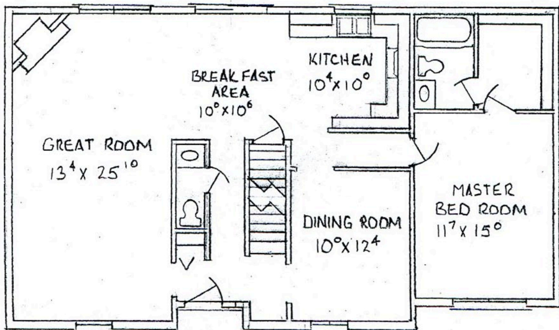
1st Floor - 1200 sq ft
